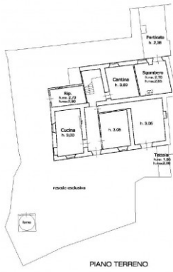
PIANO TERRENO
